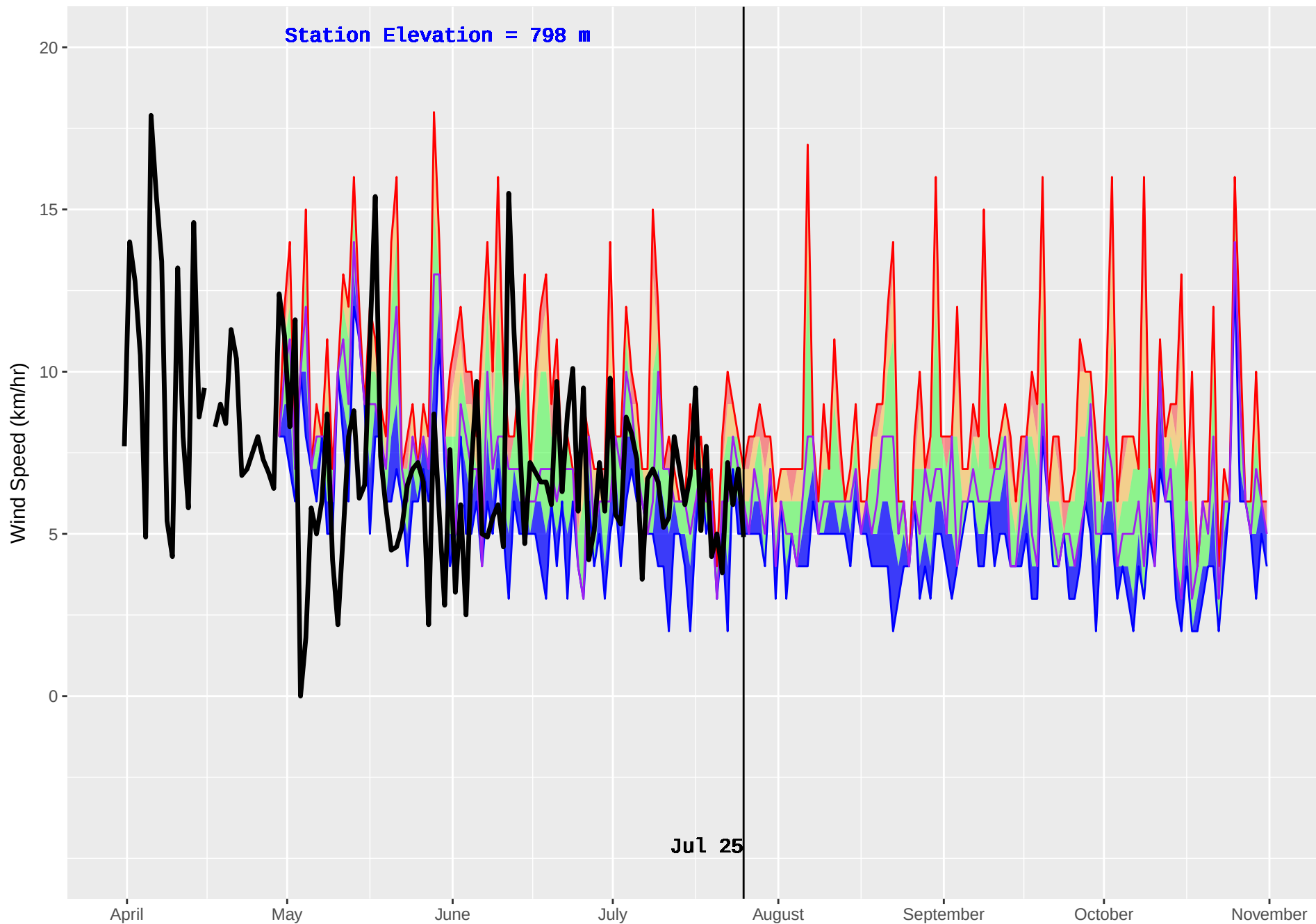
SEVEREID (1165) : Historical (2014–2016) and Current (2018) Noon Wind Speed
